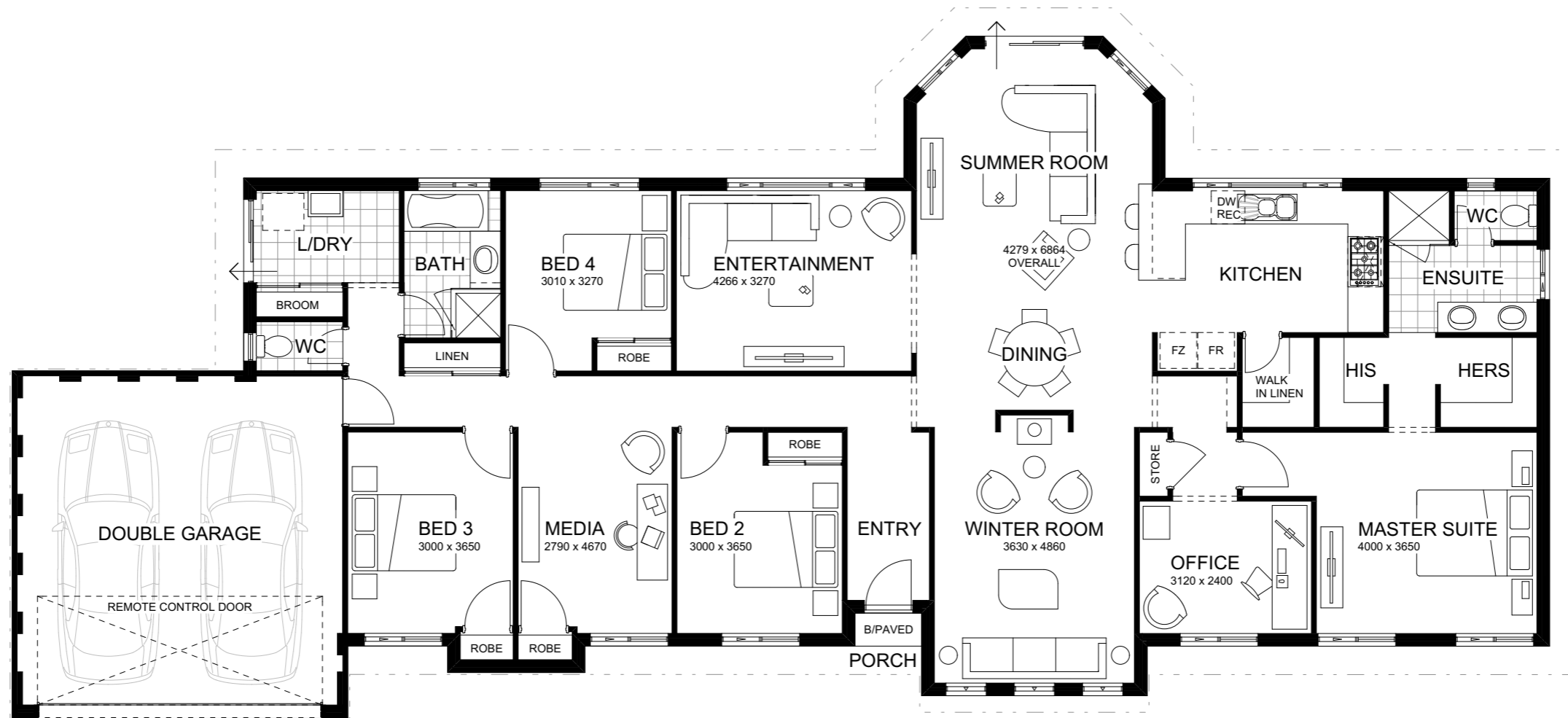
FLOOR PLAN 1:100
