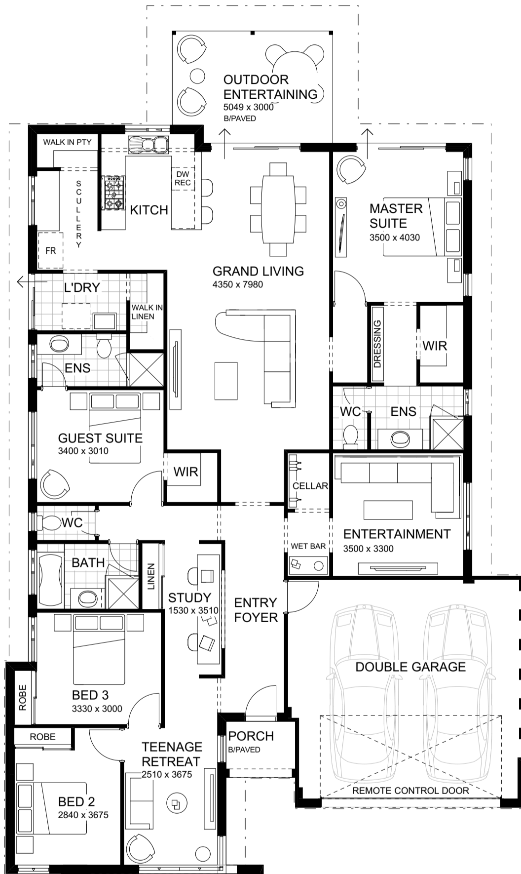
FLOOR PLAN 1:100
