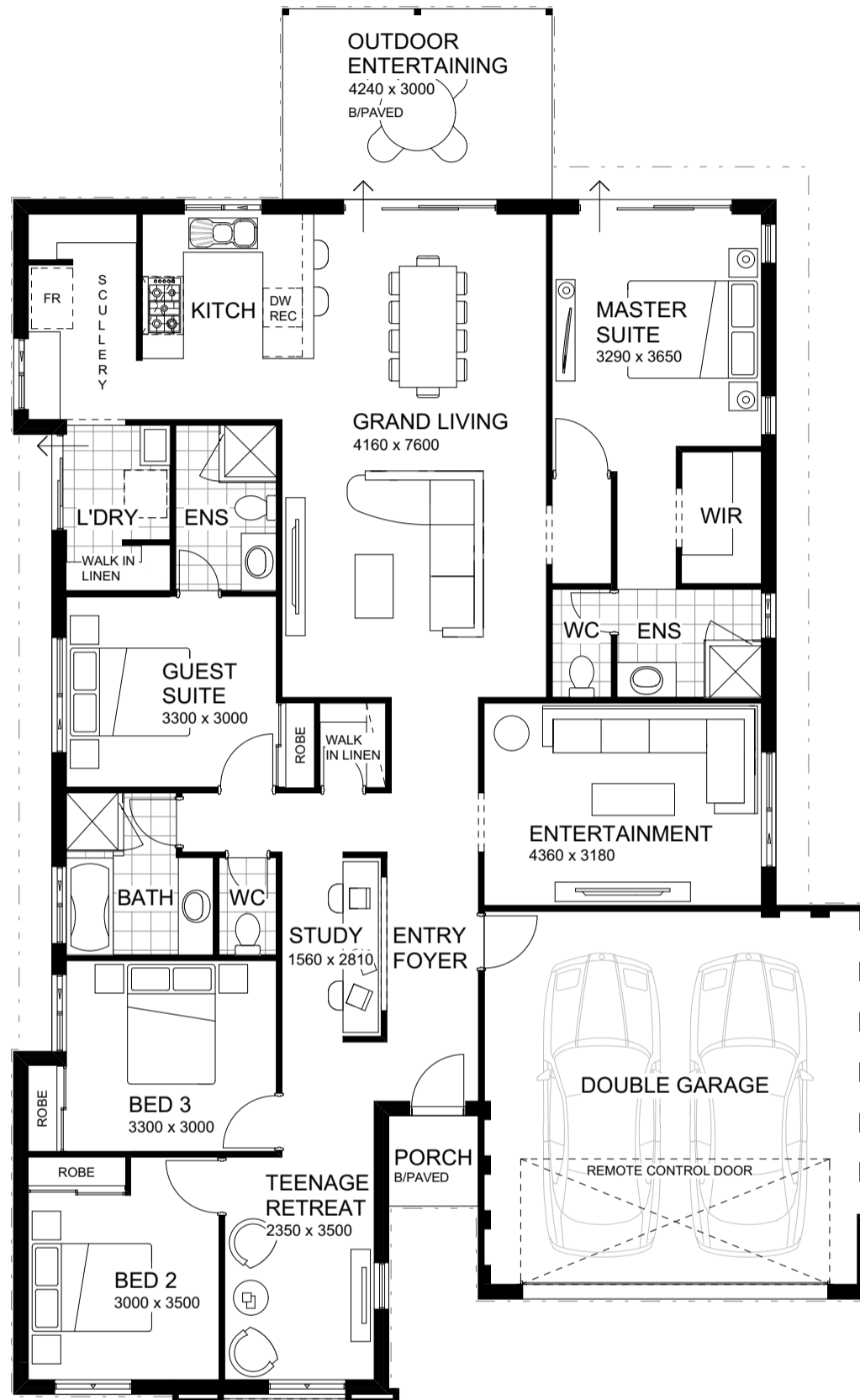
FLOOR PLAN 1:100
