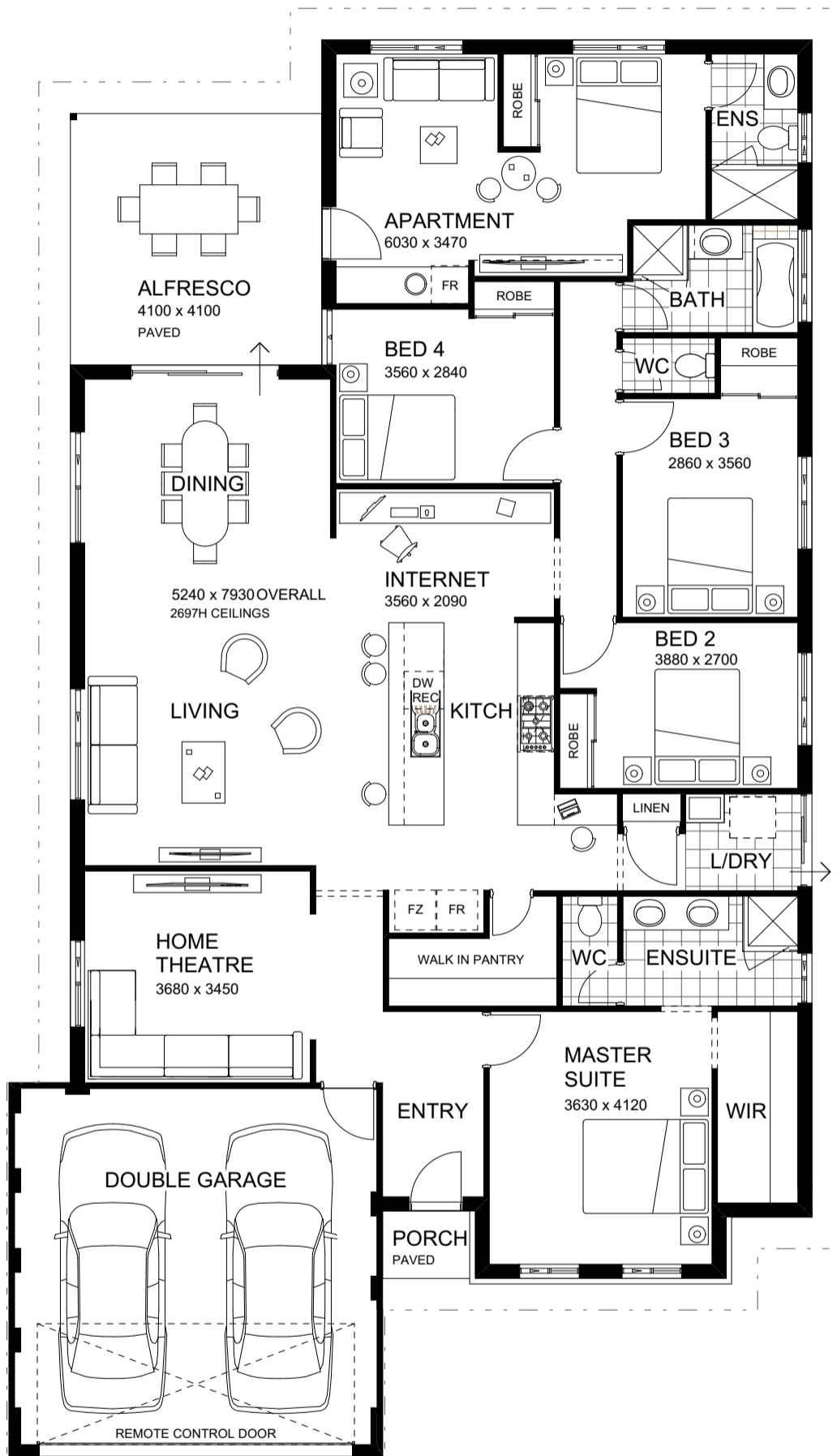
FLOOR PLAN 1:100
