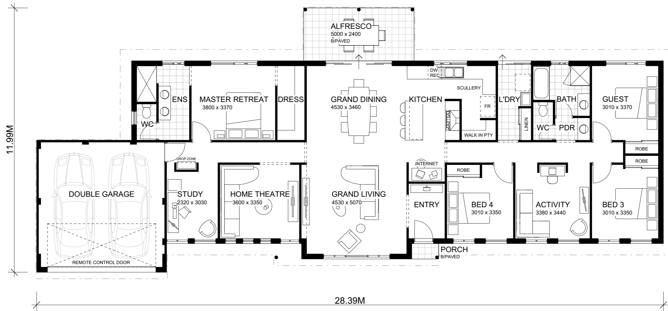
FLOOR PLAN 1:100
