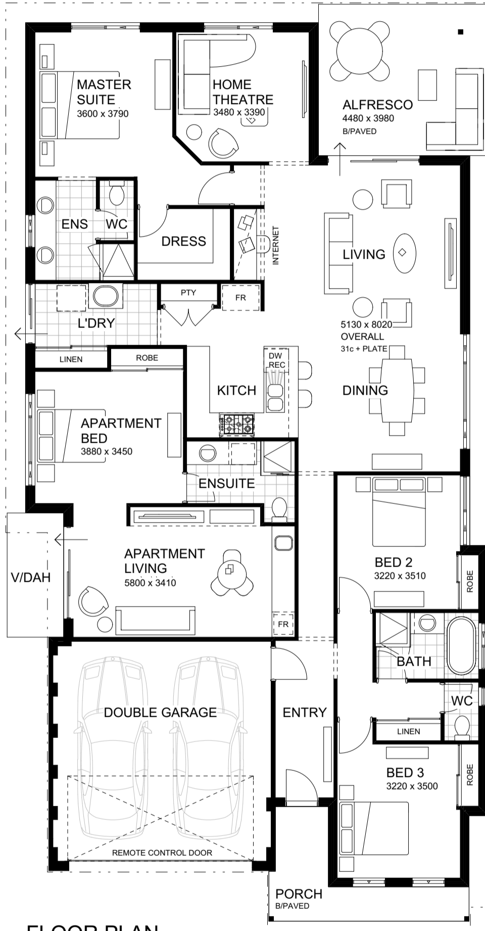
FLOOR PLAN 1:100
