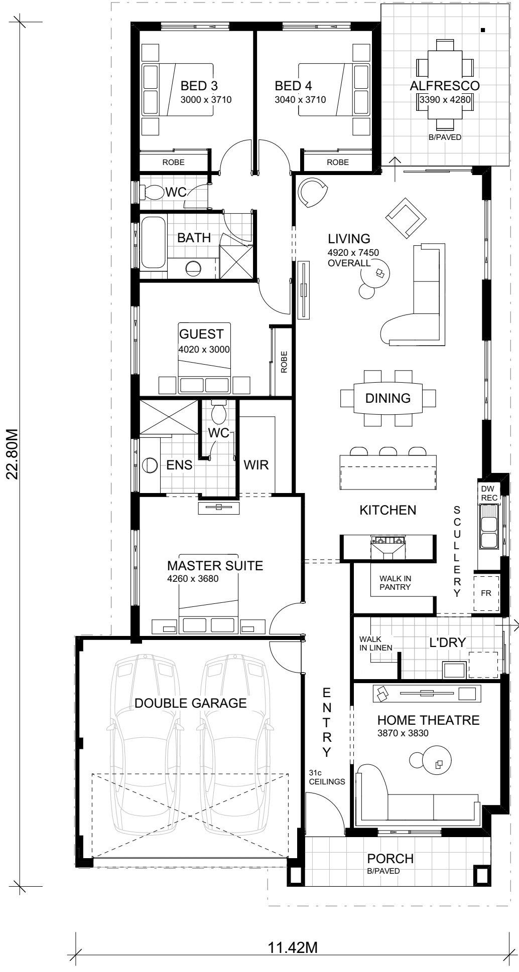
FLOOR PLAN 1:100
