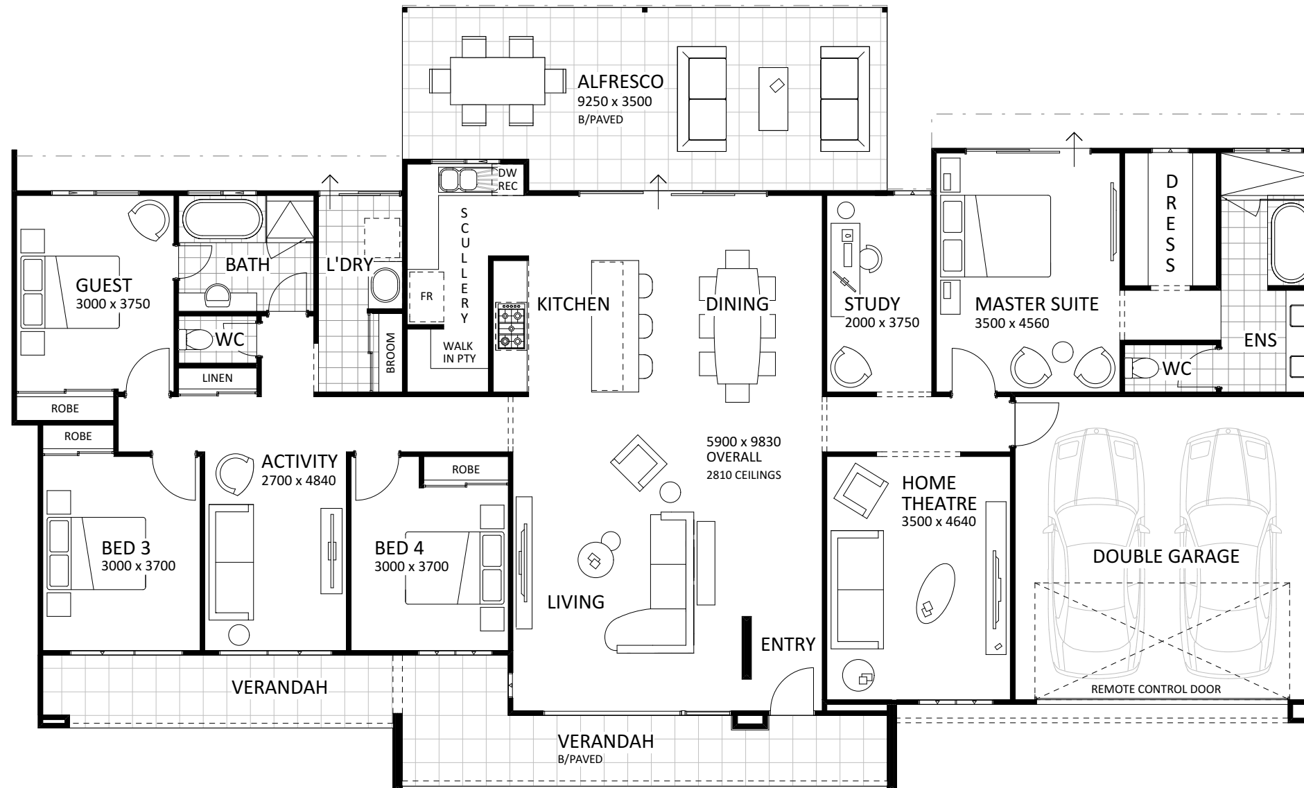
FLOOR PLAN 1:100
