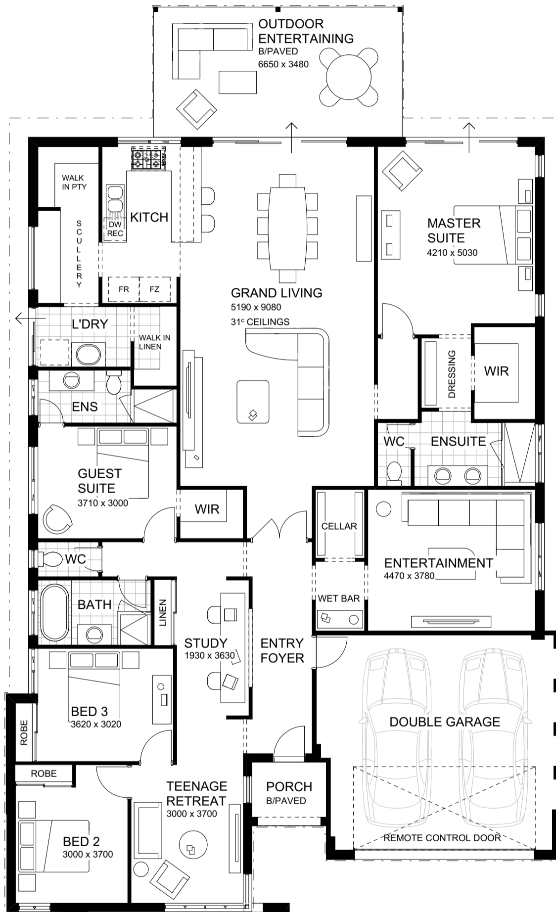
FLOOR PLAN 1:100
