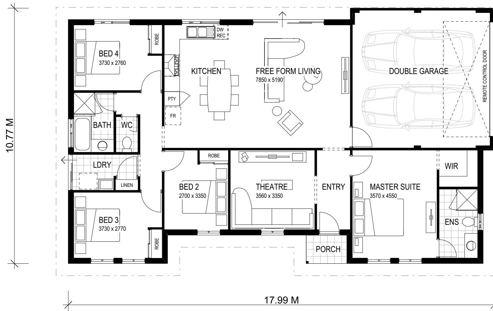
FLOOR PLAN 1:100
