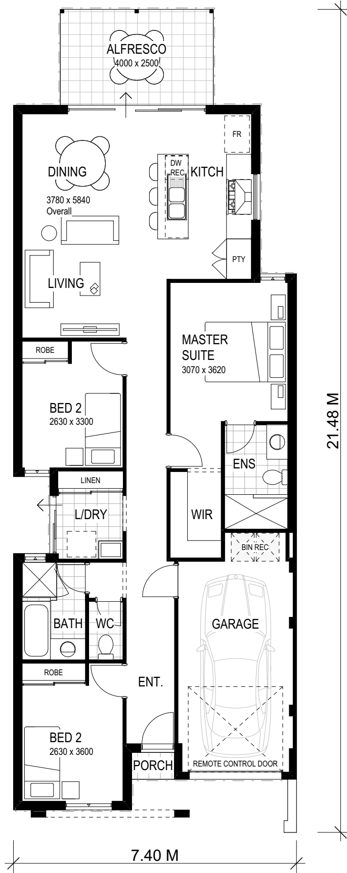
FLOOR PLAN 1:100
