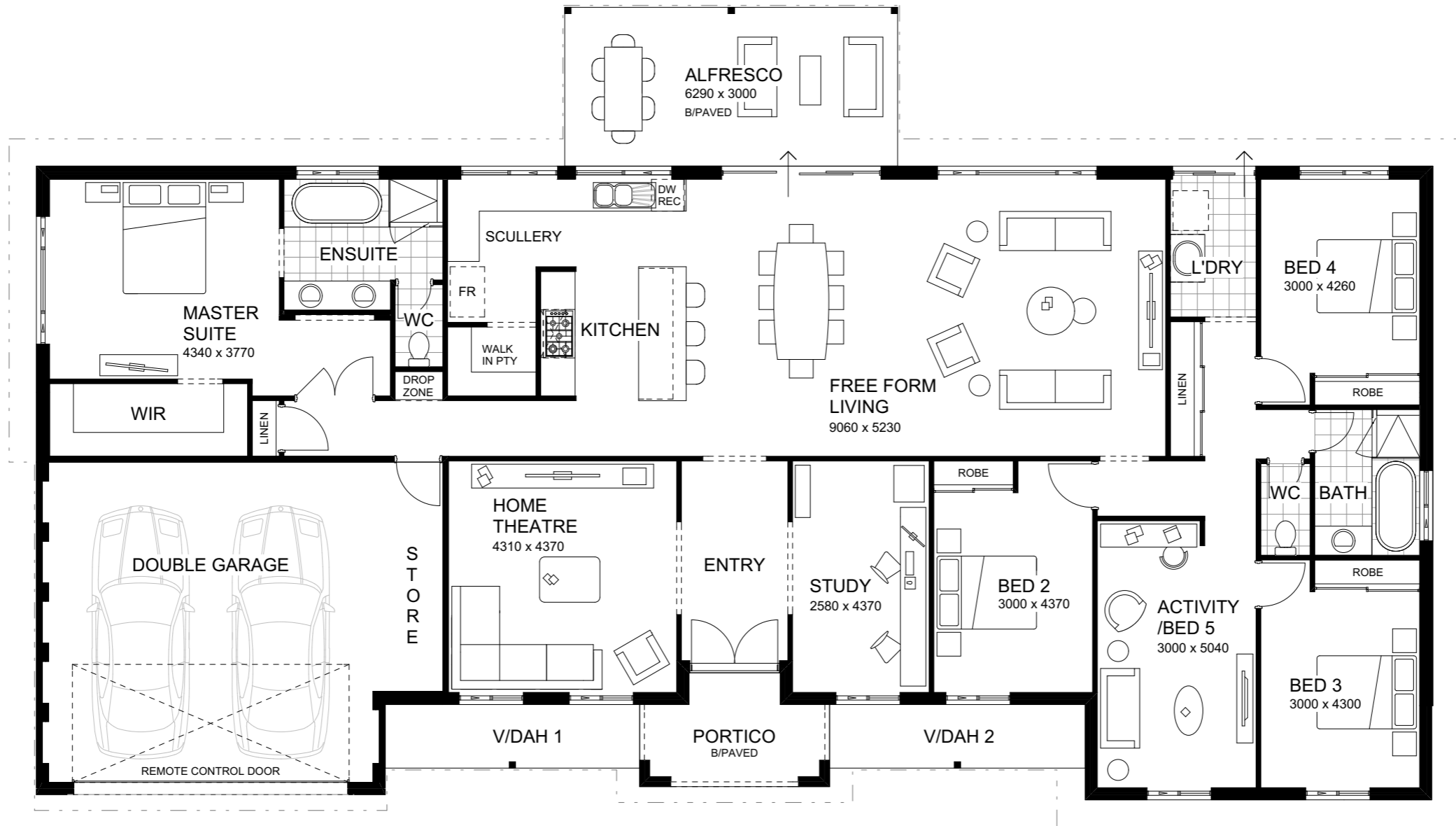
FLOOR PLAN 1:100
