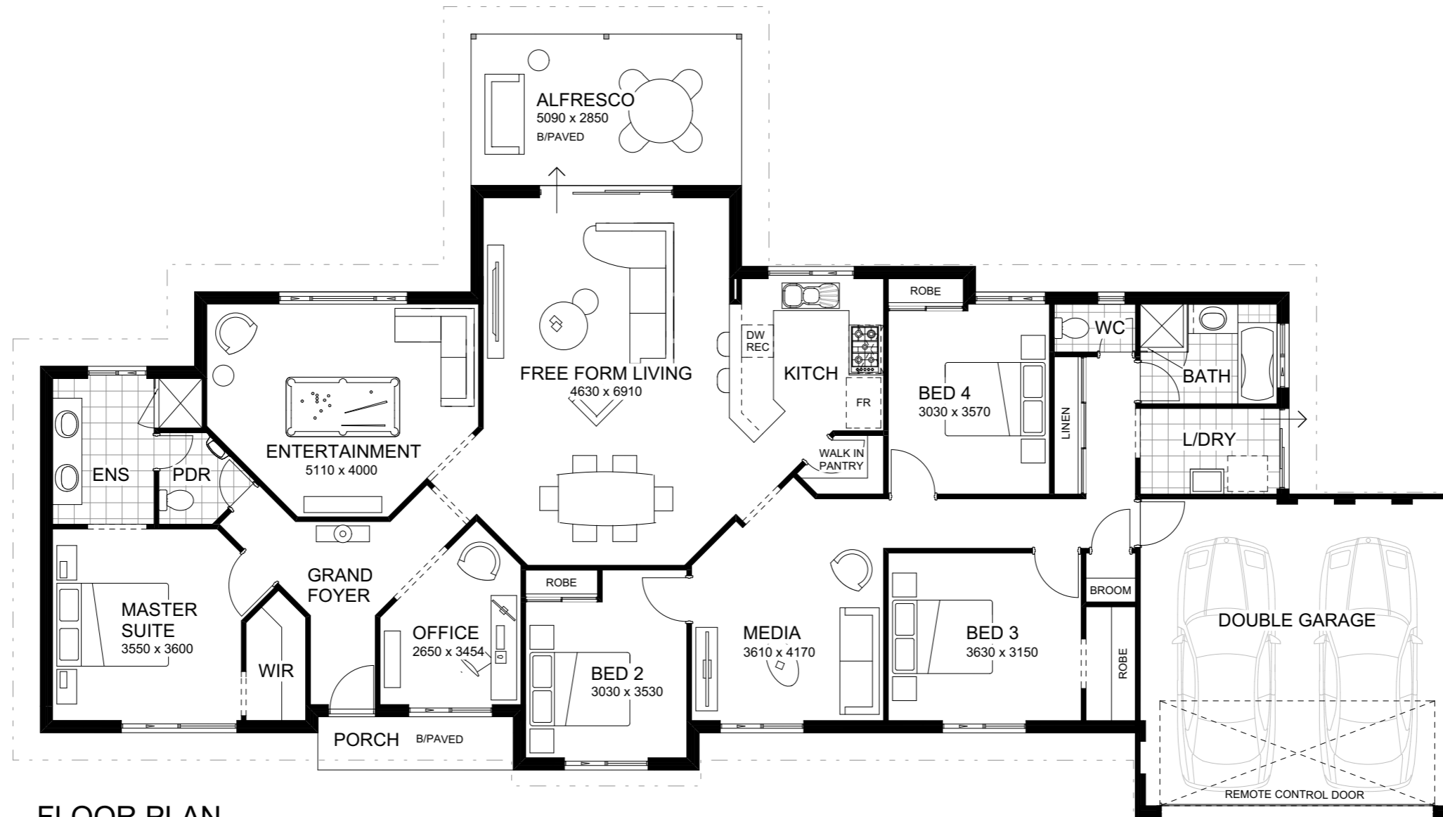
FLOOR PLAN 1:100
