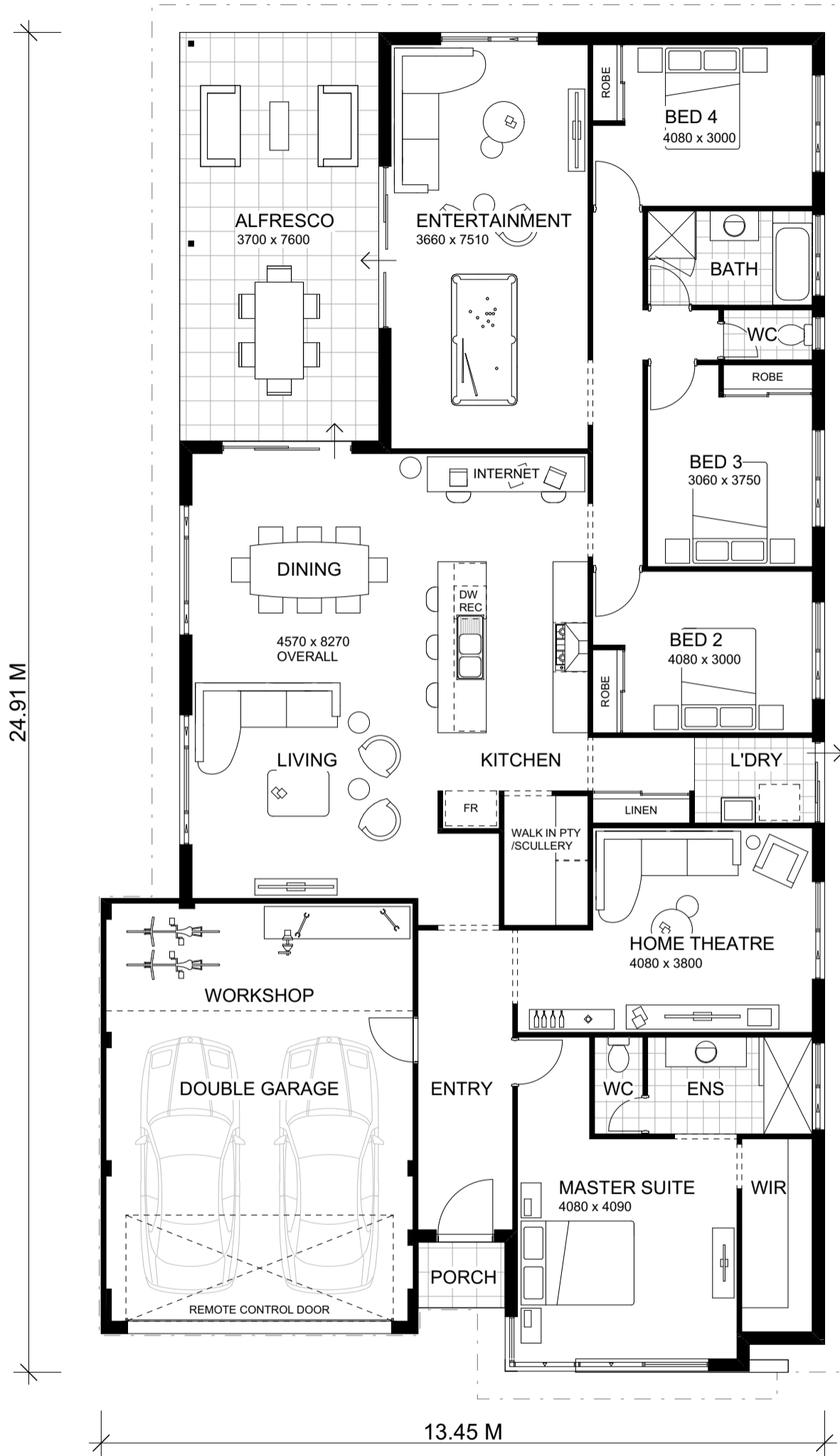
FLOOR PLAN 1:100
