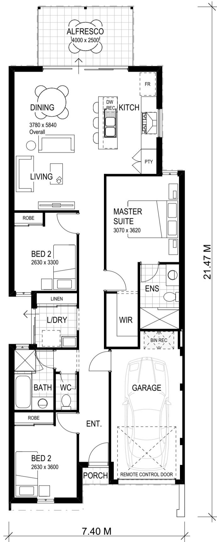
FLOOR PLAN 1:100
