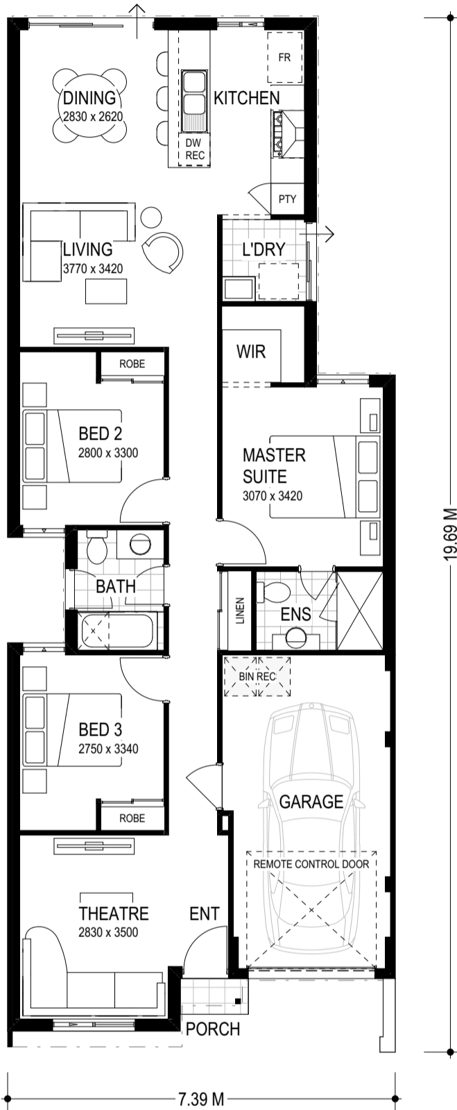
FLOOR PLAN 1:100
