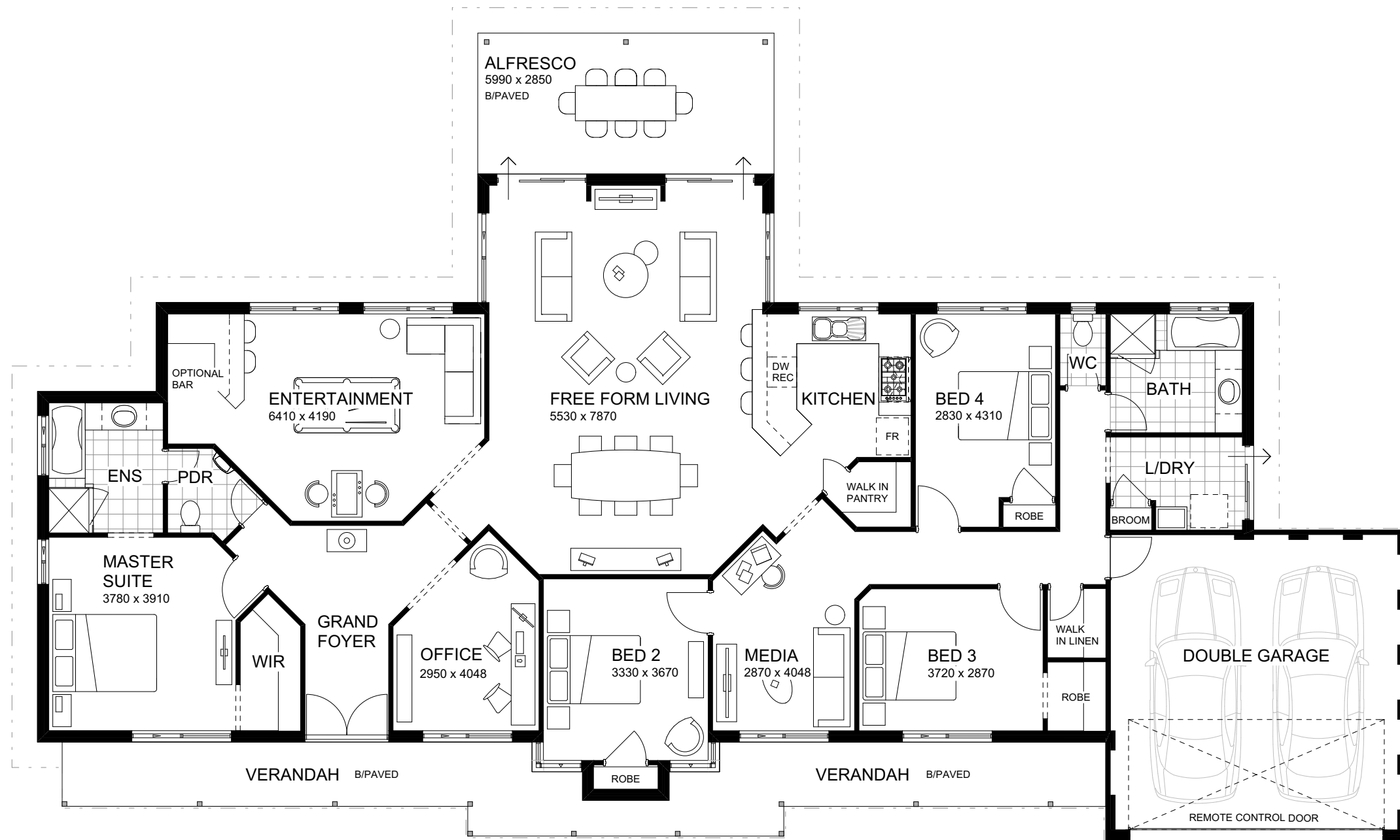
FLOOR PLAN 1:100
