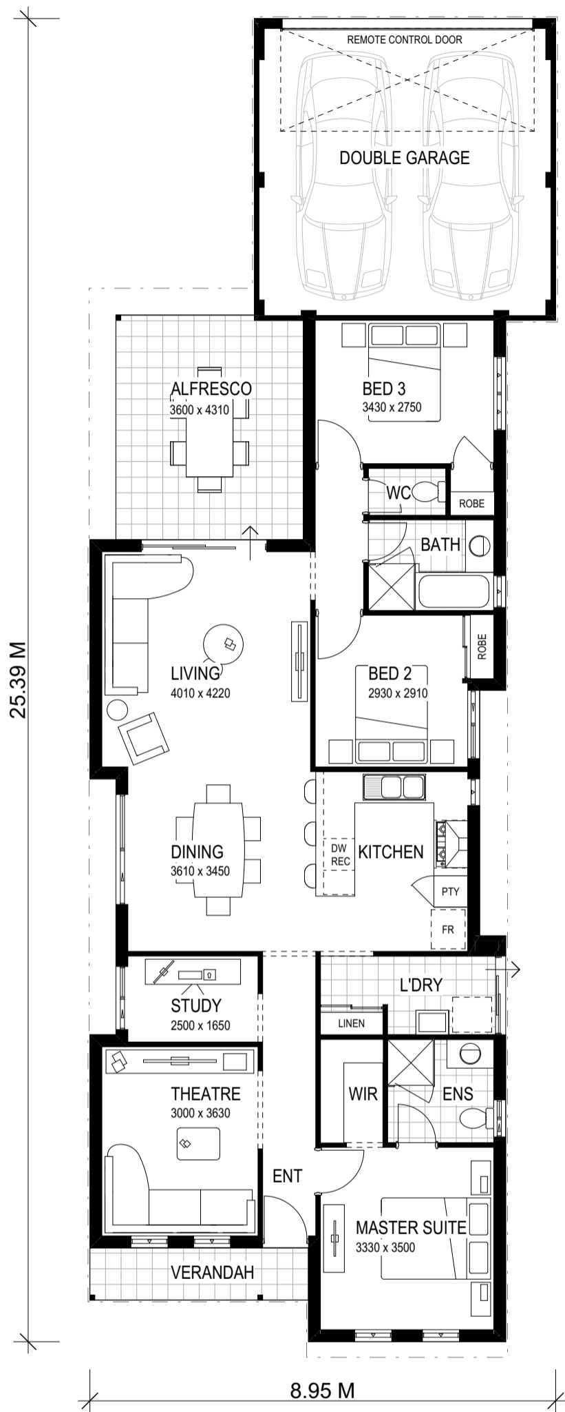
FLOOR PLAN 1:100
