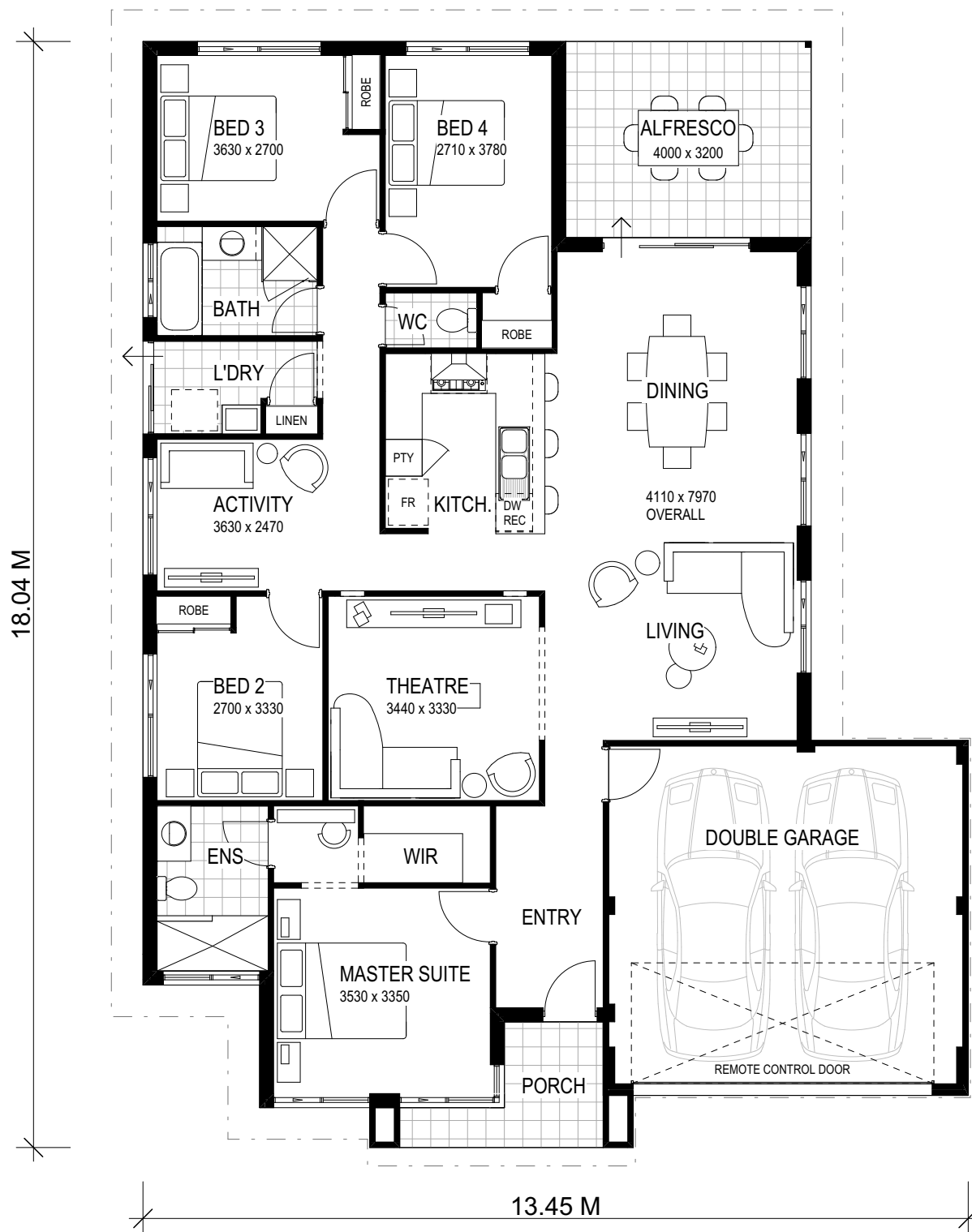
FLOOR PLAN 1:100
