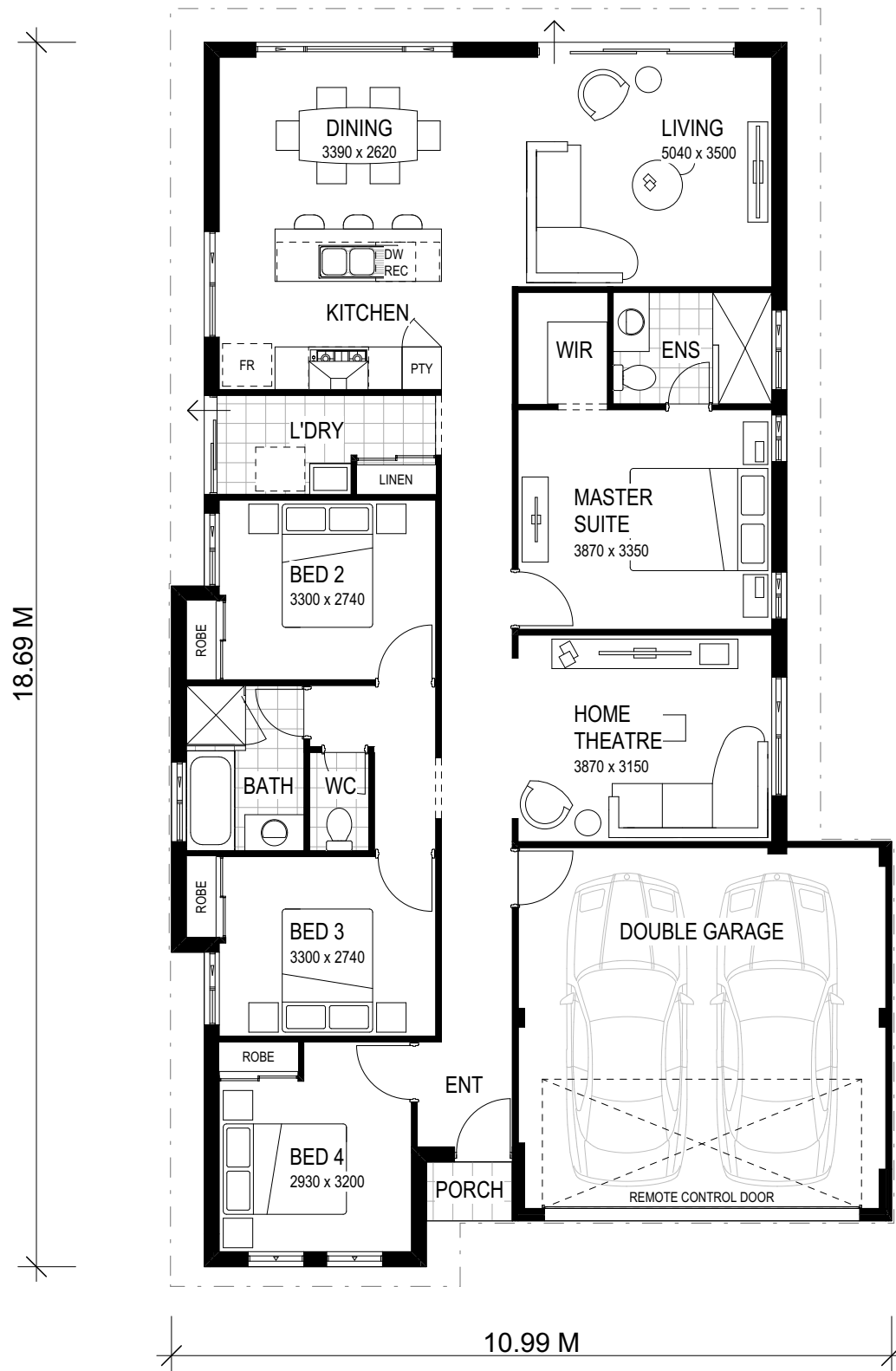
FLOOR PLAN 1:100
