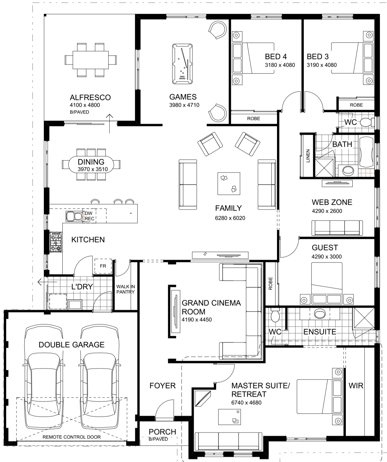
FLOOR PLAN 1:100
