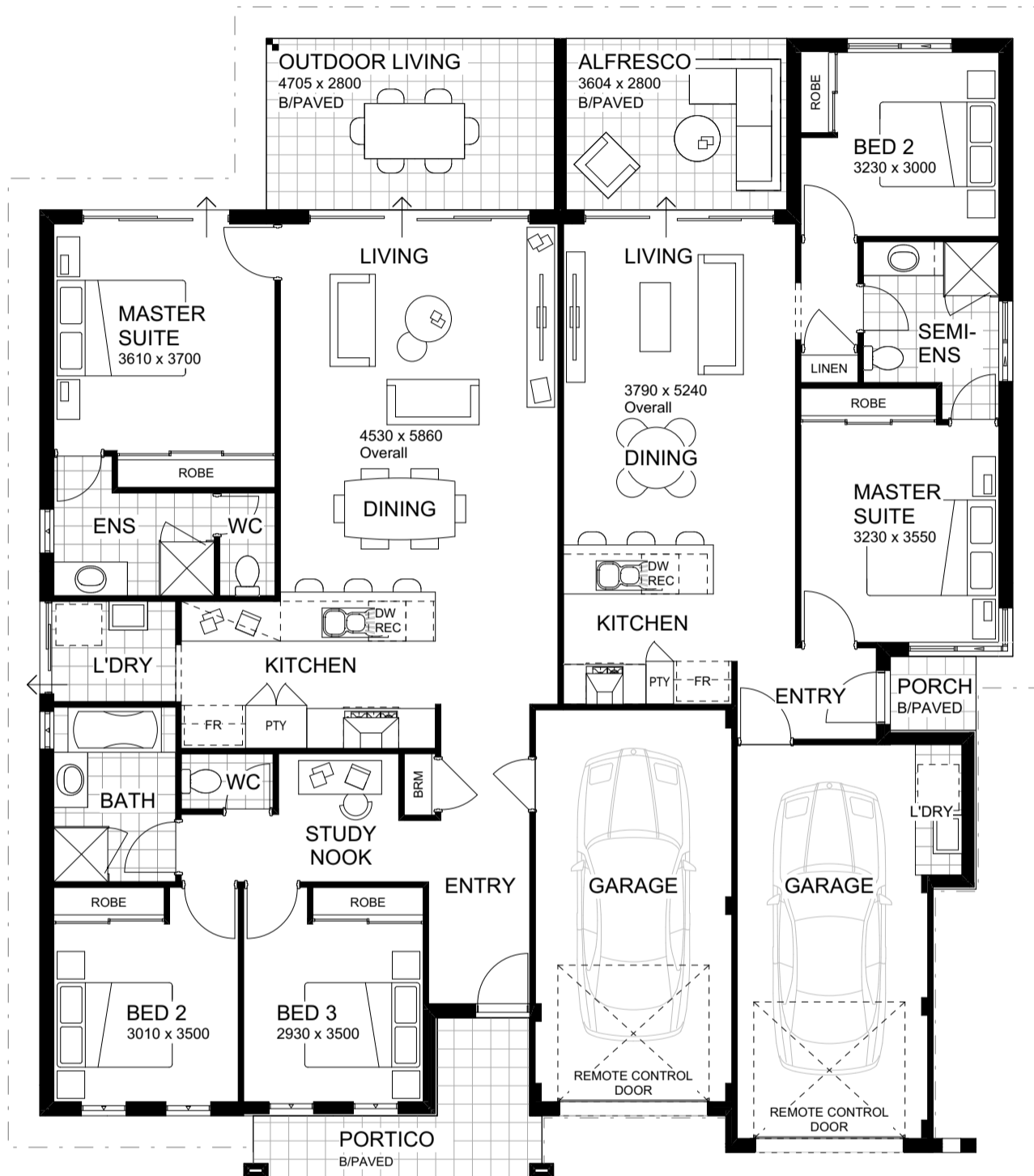
FLOOR PLAN 1:100
