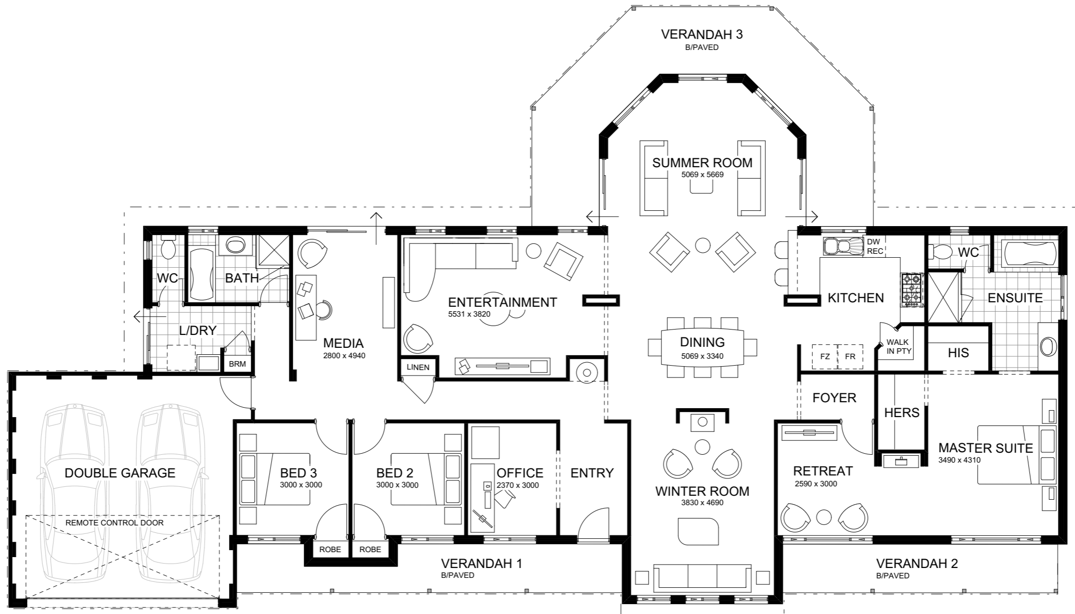
FLOOR PLAN 1:100
