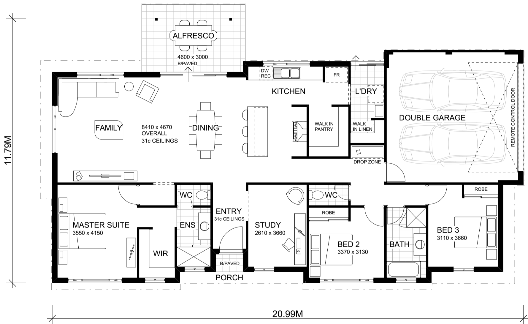
FLOOR PLAN 1:100
