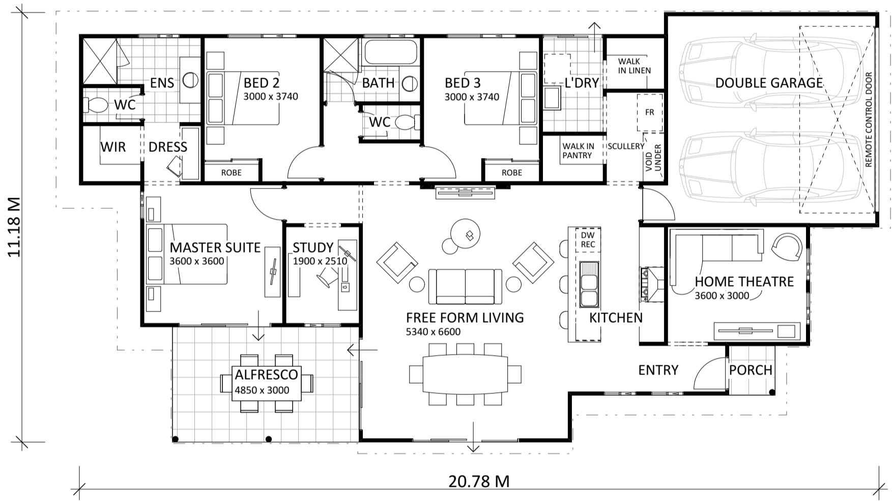
FLOOR PLAN 1:100
