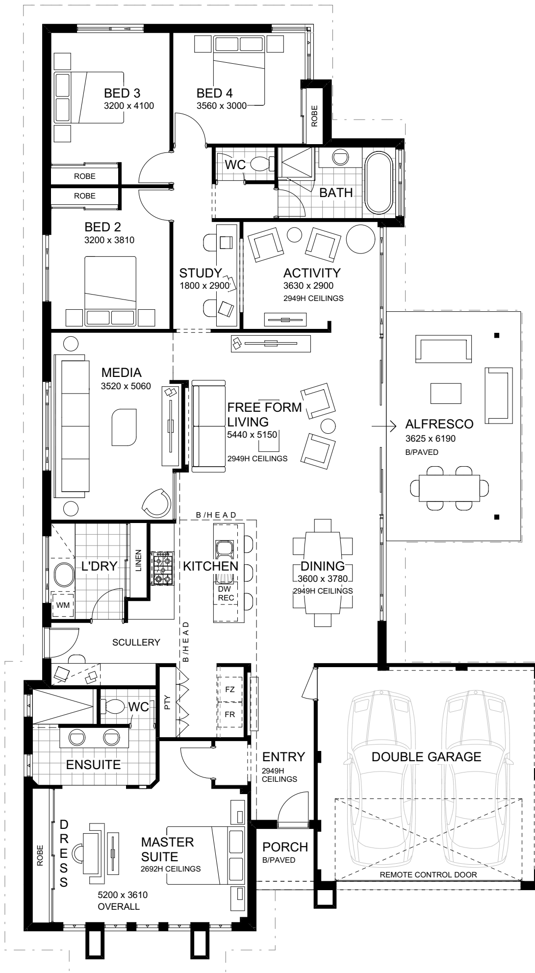
FLOOR PLAN 1:100
