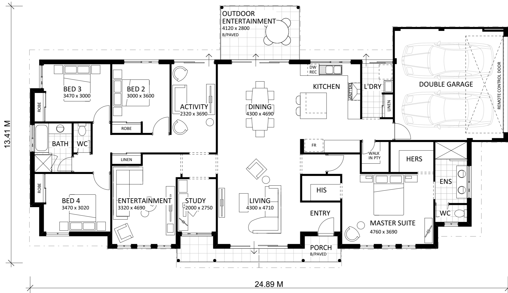
FLOOR PLAN 1:100
