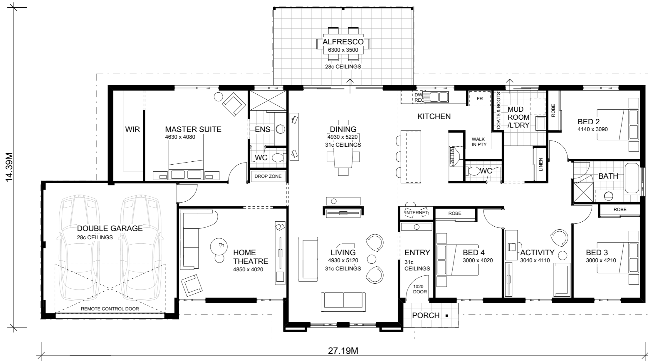
FLOOR PLAN 1:100
