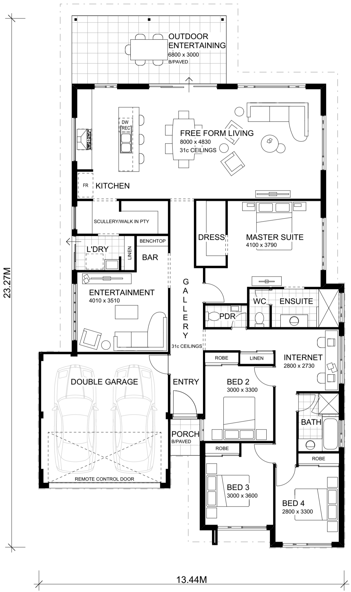
FLOOR PLAN 1:100
