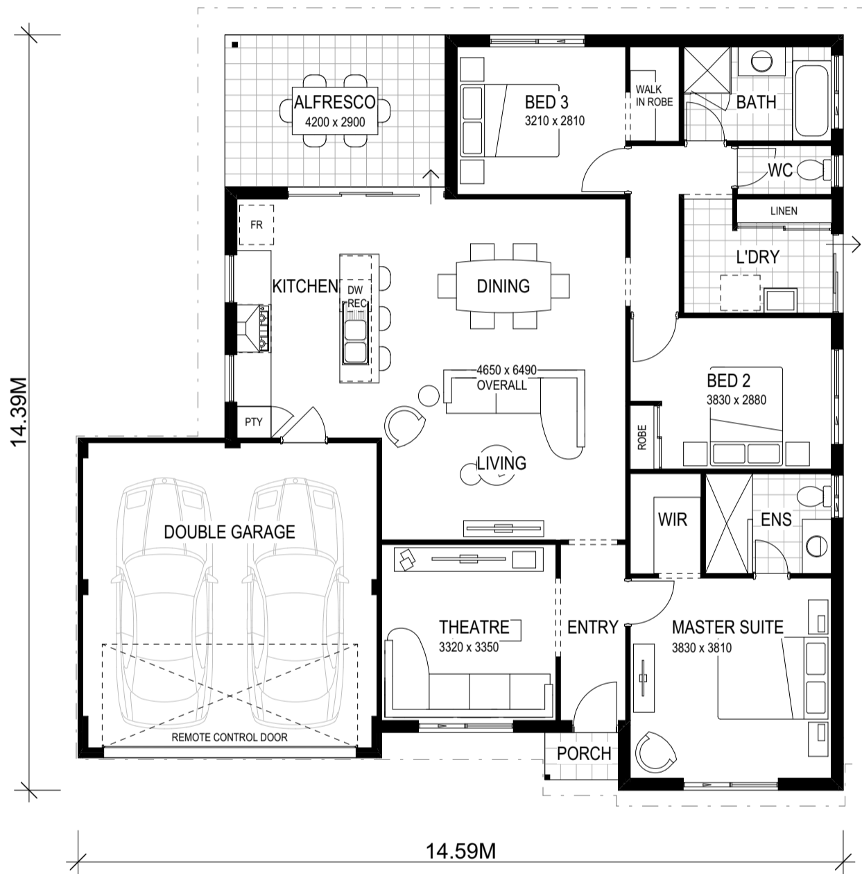
FLOOR PLAN 1:100
