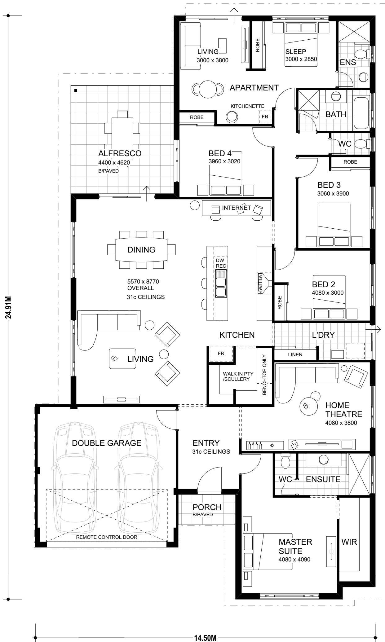
FLOOR PLAN 1:100
