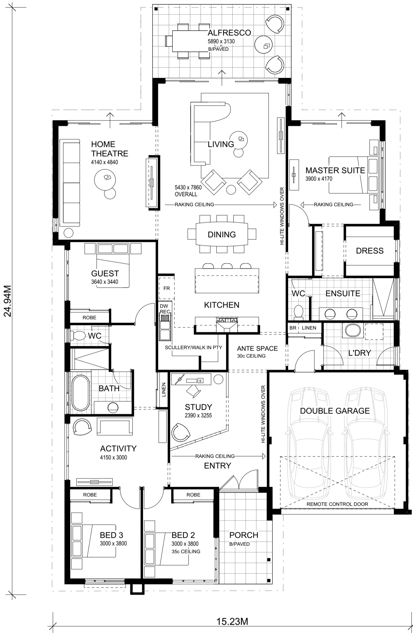
FLOOR PLAN 1:100
