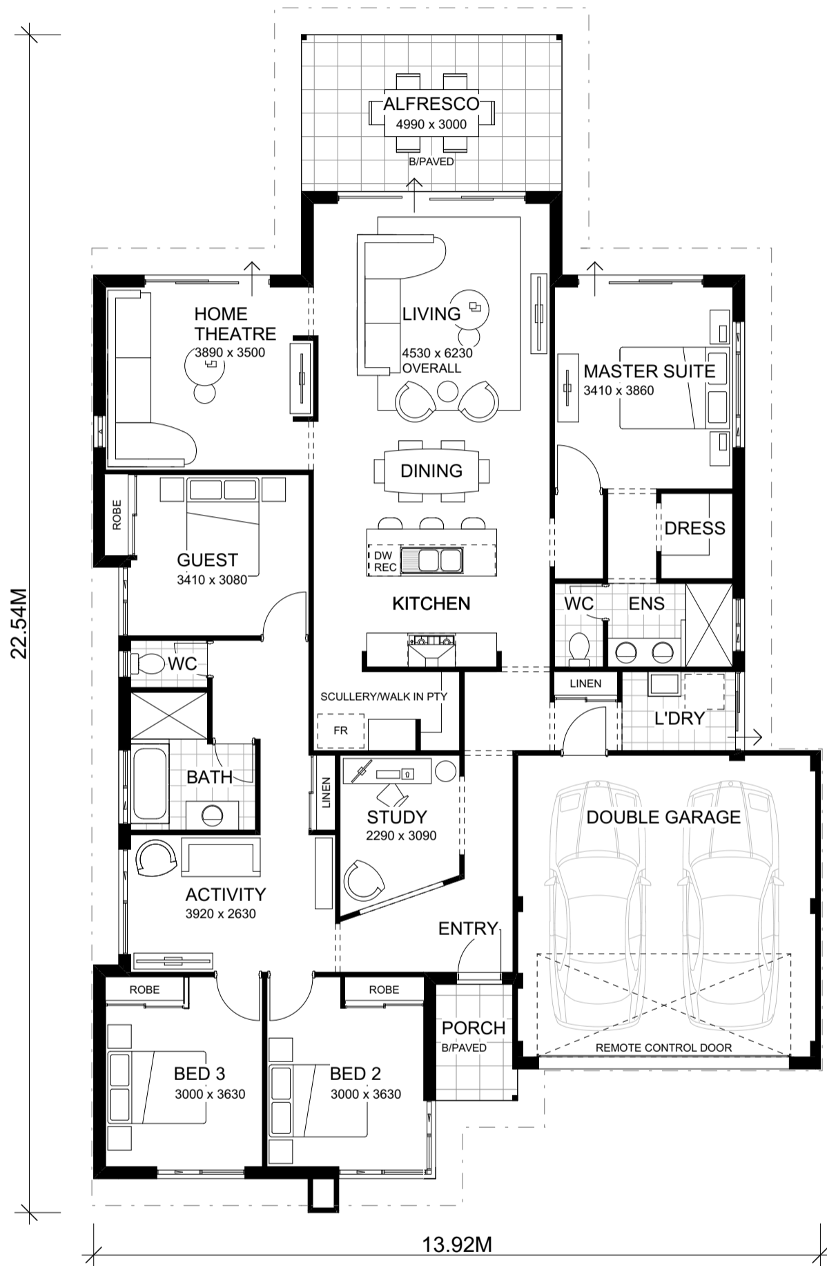
FLOOR PLAN 1:100
