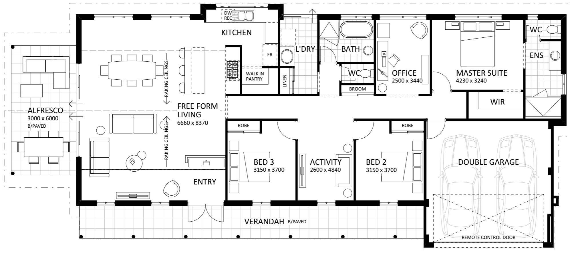
FLOOR PLAN 1:100
