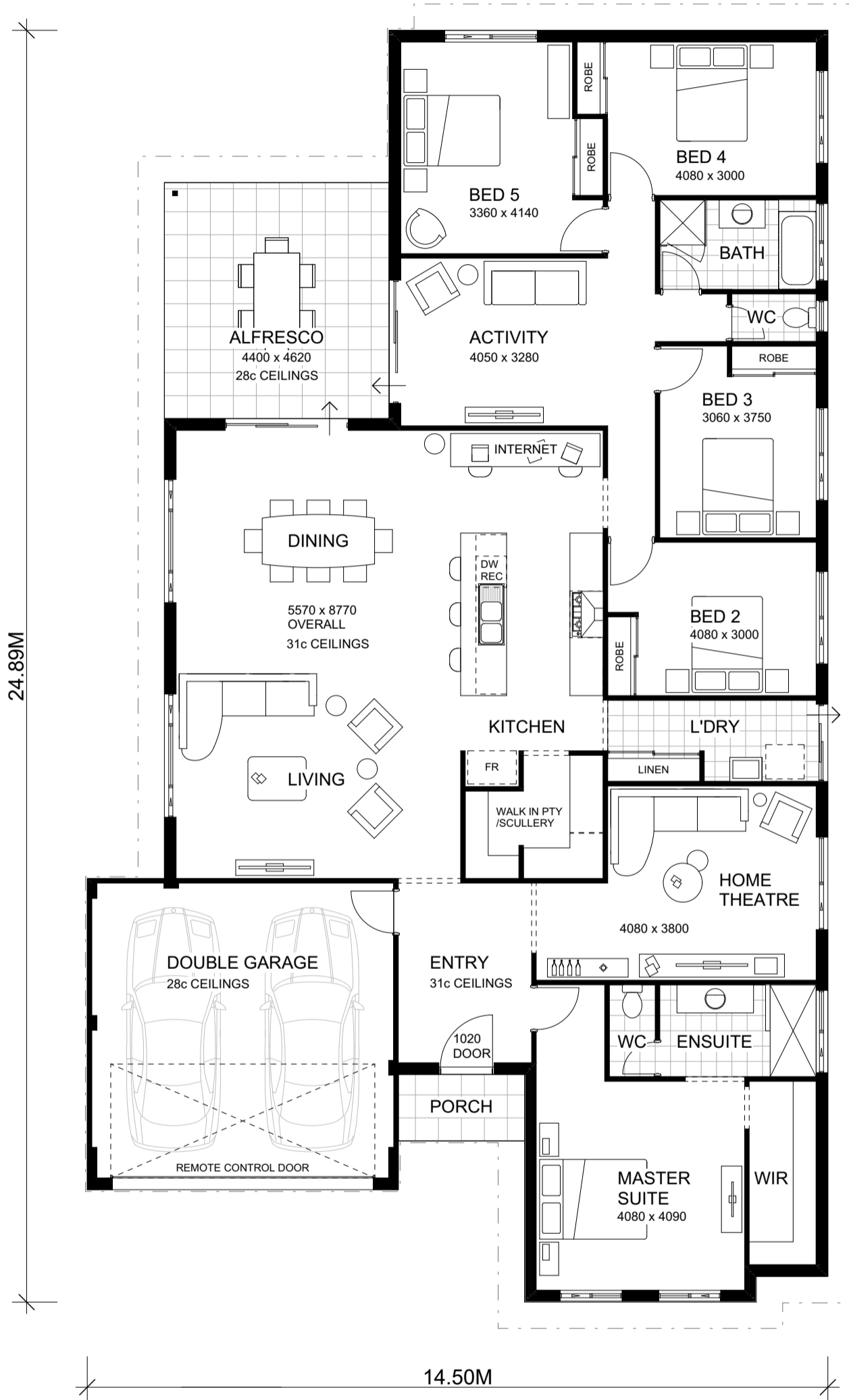
FLOOR PLAN 1:100
