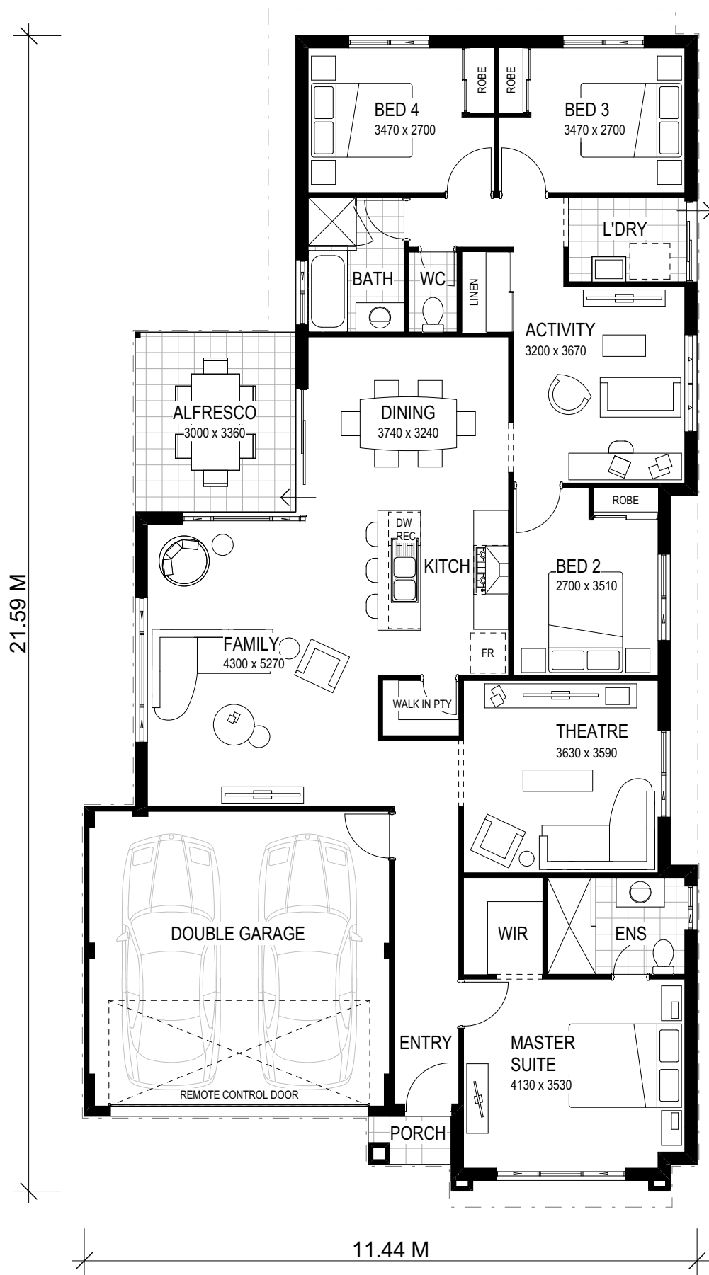
FLOOR PLAN 1:100
