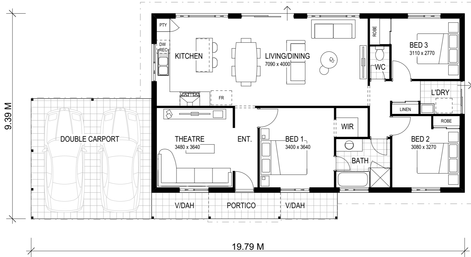
FLOOR PLAN 1:100
