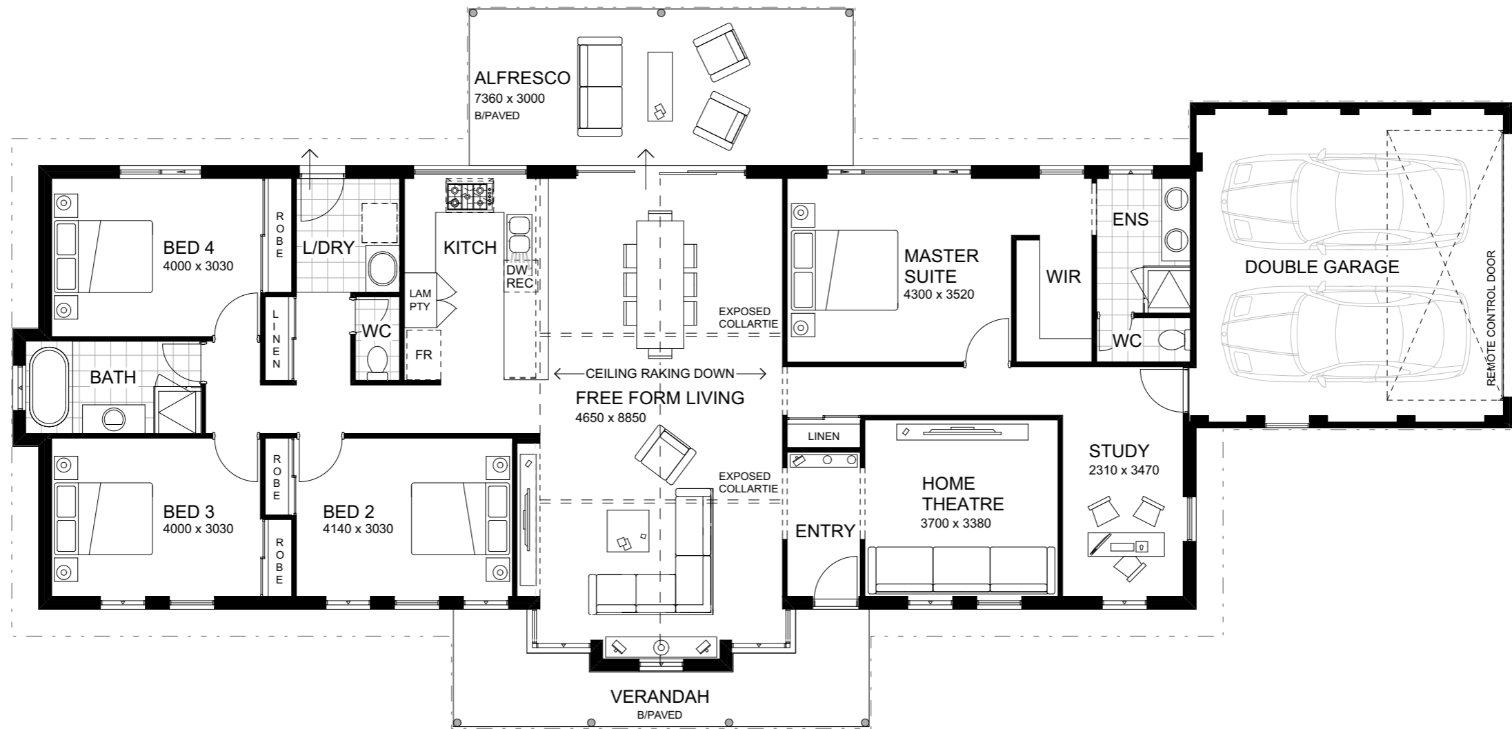
FLOOR PLAN 1:100
