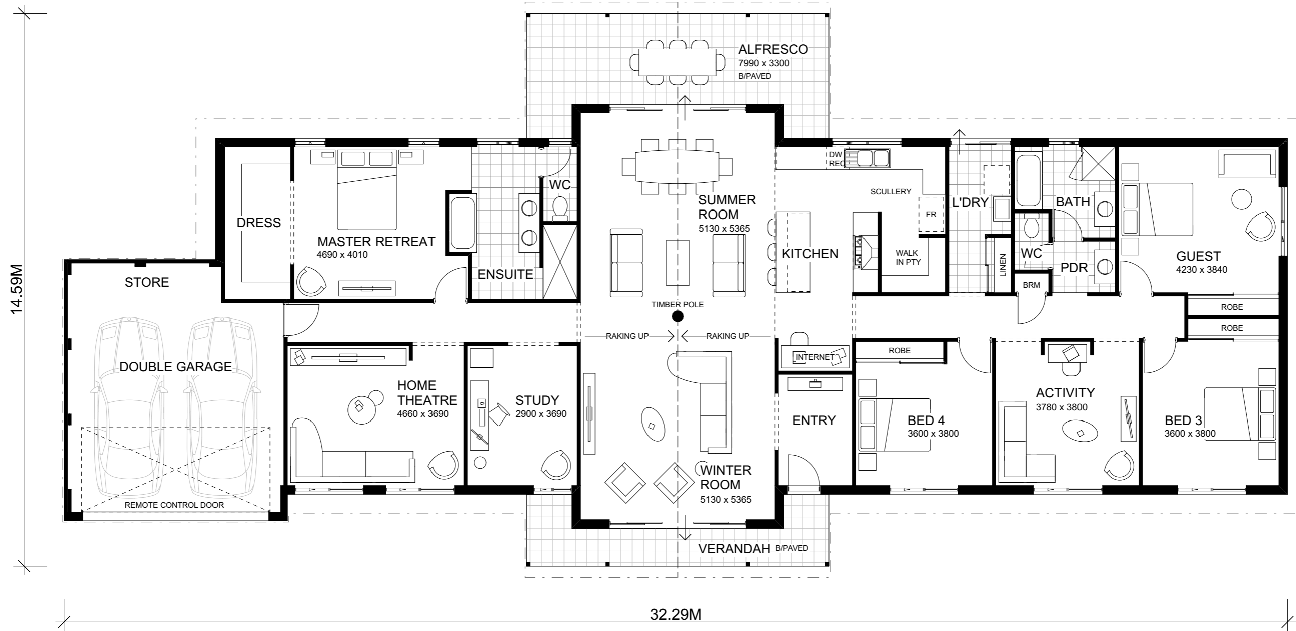
FLOOR PLAN 1:100
