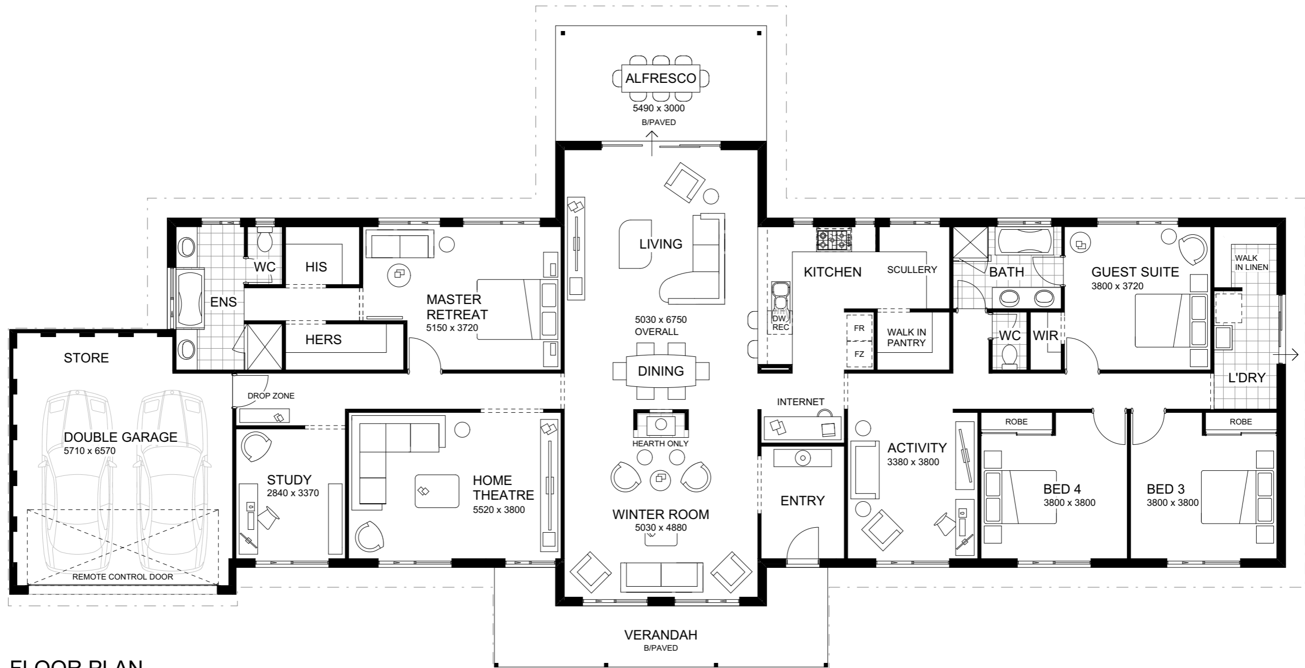
FLOOR PLAN 1:100
