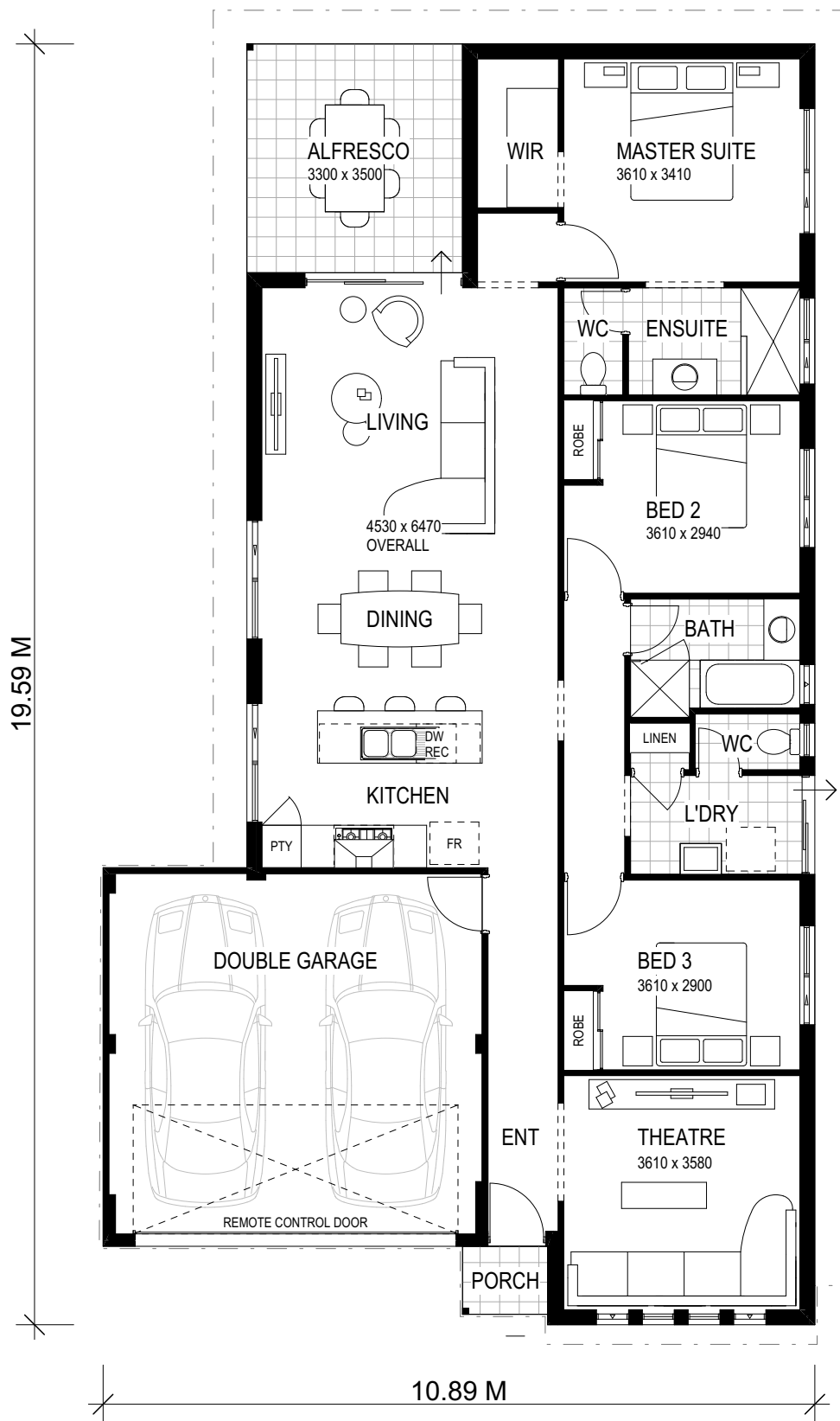
FLOOR PLAN 1:100
