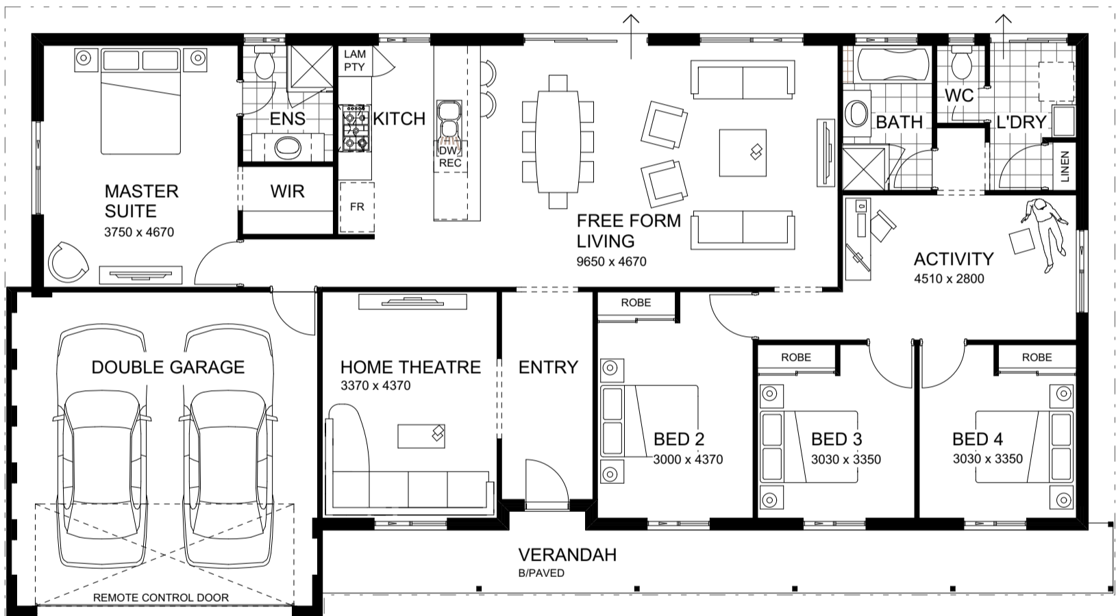
FLOOR PLAN 1:100
