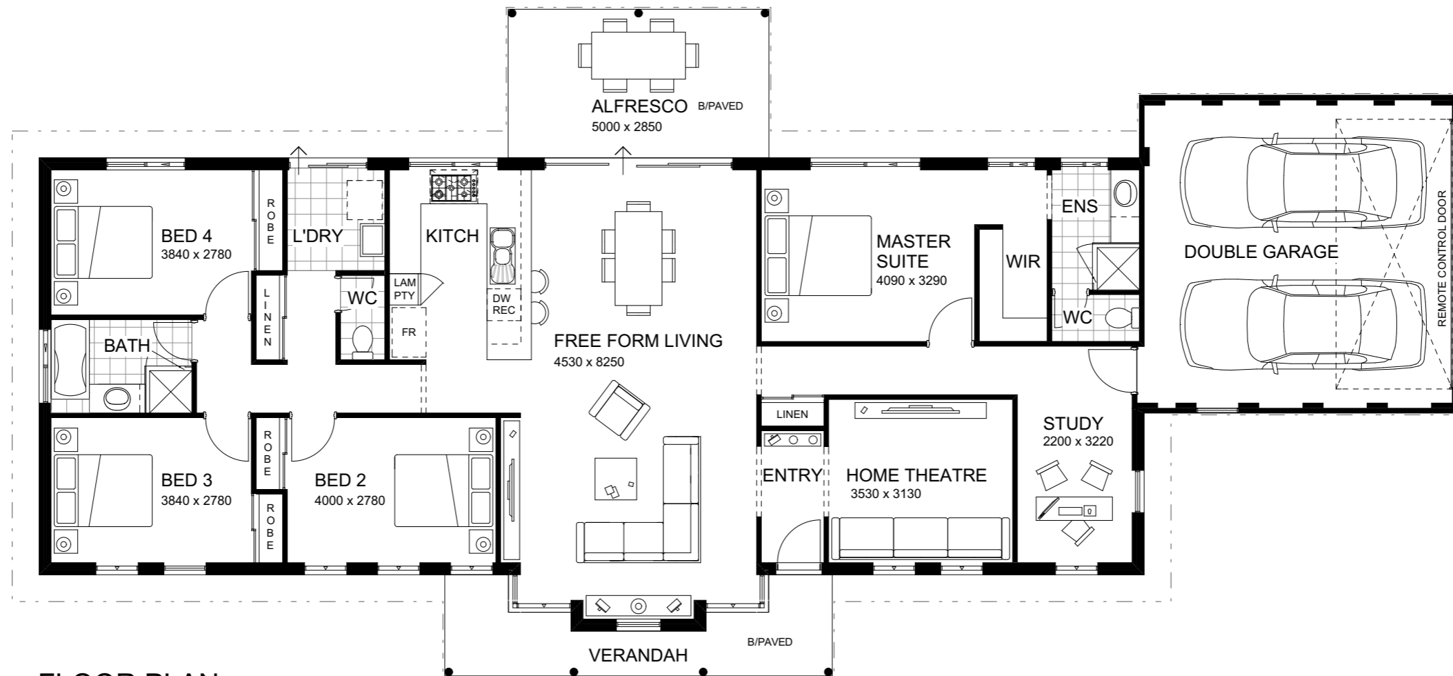
FLOOR PLAN 1:100
