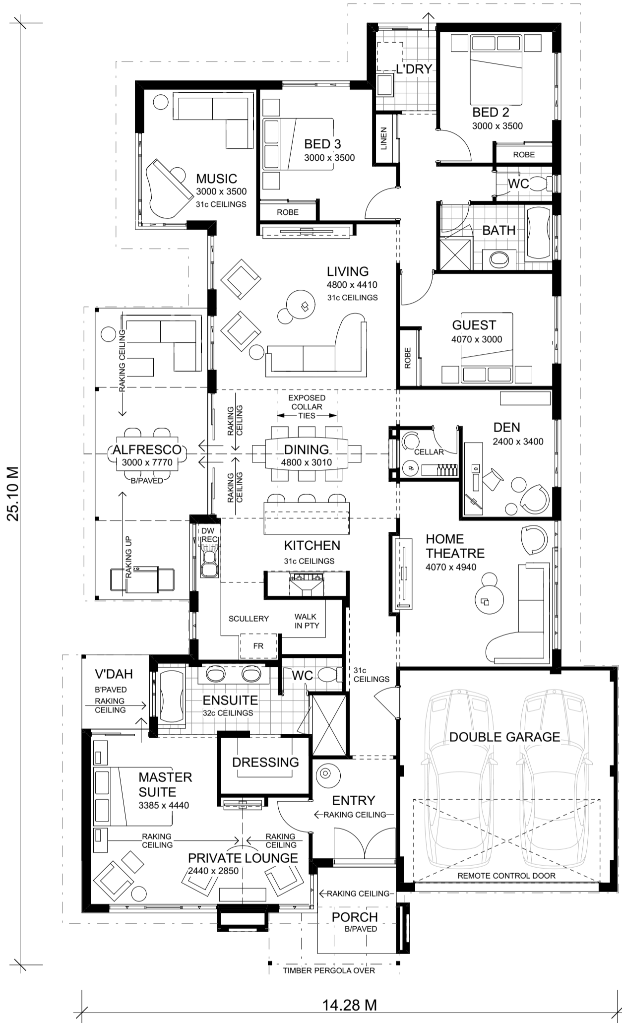
FLOOR PLAN 1:100
