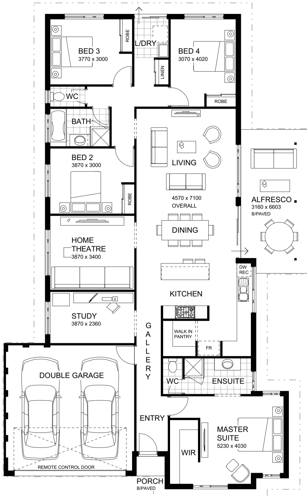
FLOOR PLAN 1:100
