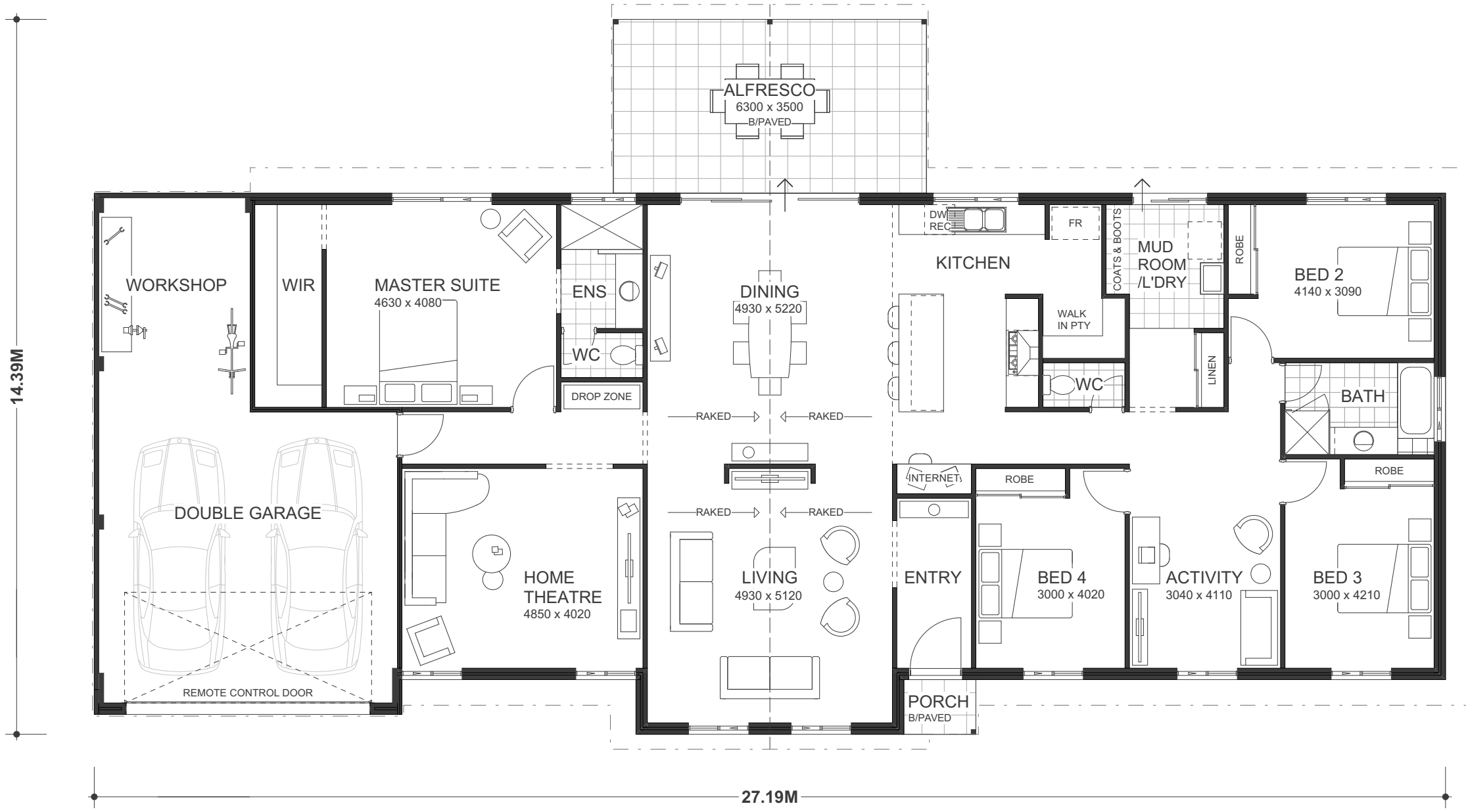
FLOOR PLAN 1:100
